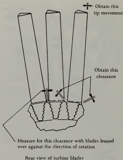
FIGURE 10-64. Turbine blade replacement clearances.
